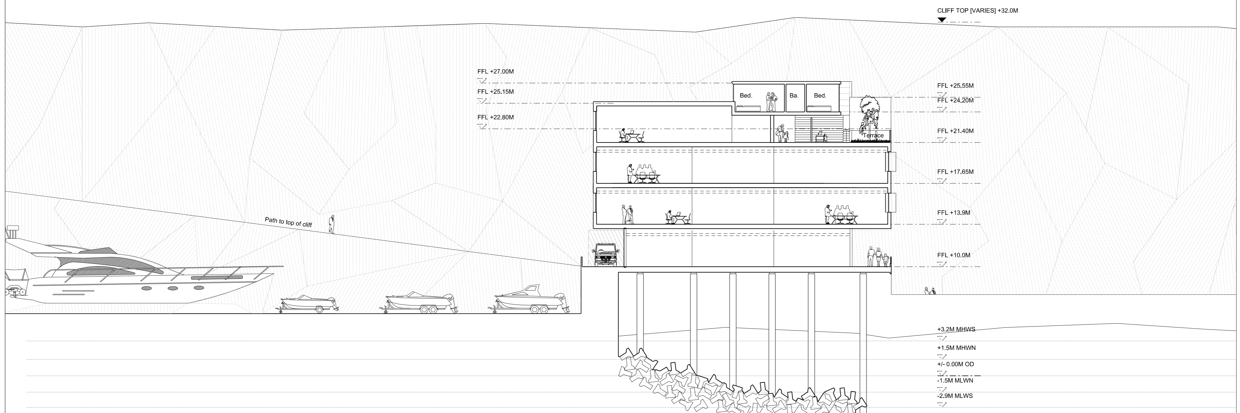
Section B - B 1:200
